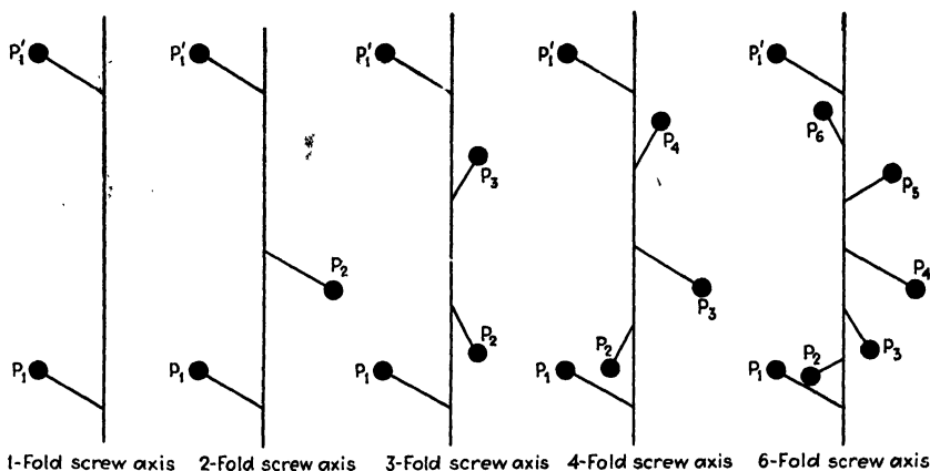
1-Fold screw axis 2-Fold screw axis 3-Fold screw axis 4-Fold screw axis 6-Fold screw axis FIG. 3.—Perspective view of the action of 1-fold, 2-fold, 3-fold, 4-fold, and 6-fold screw axes. Point-groups C_1 , C_2 , C_3 , C_4 , C_6 .
